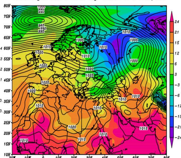
airtemperature and slp 4nov1972 surface
