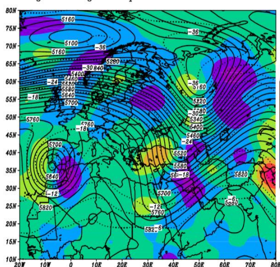
omega700&amp;hgt&amp;temperature500hPa 4nov1972
