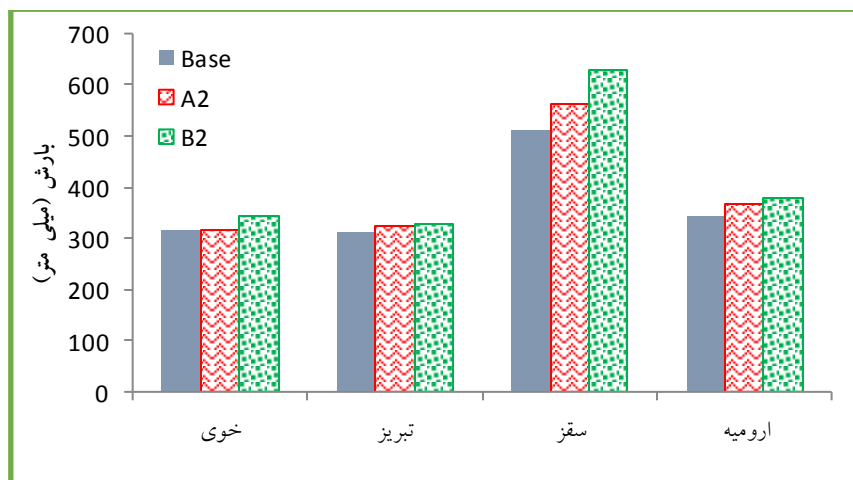
Figure 4: The state of rainfall changes in the decade (2020) compared to the base period
