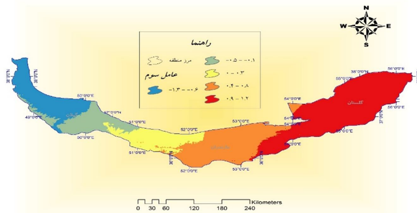
Figure 6: Spatial pattern of the second factor in the region (humidity and precipitation factor)
