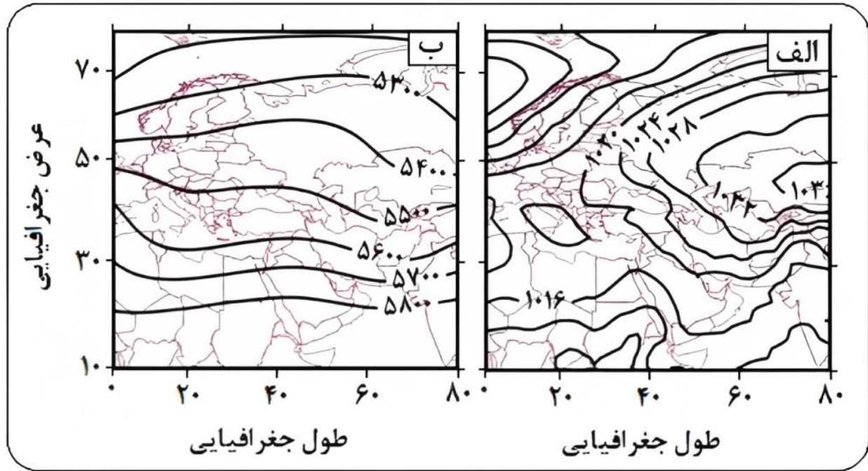
Figure 6: a) Average Sea level pressure (hectopascals), b) Average level height of 500 hectopascals (geopotential meters) for the third pattern
